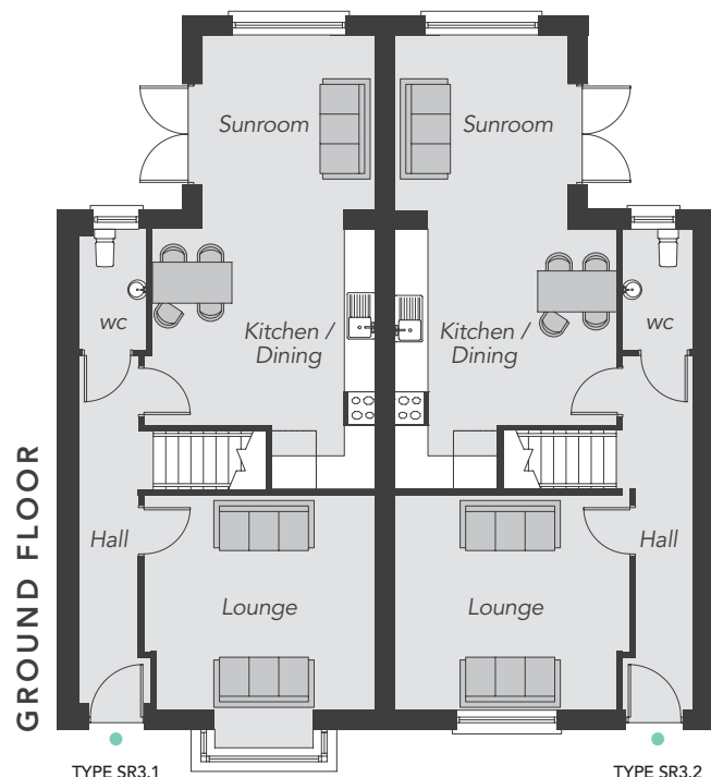
TYPE SR3.1
